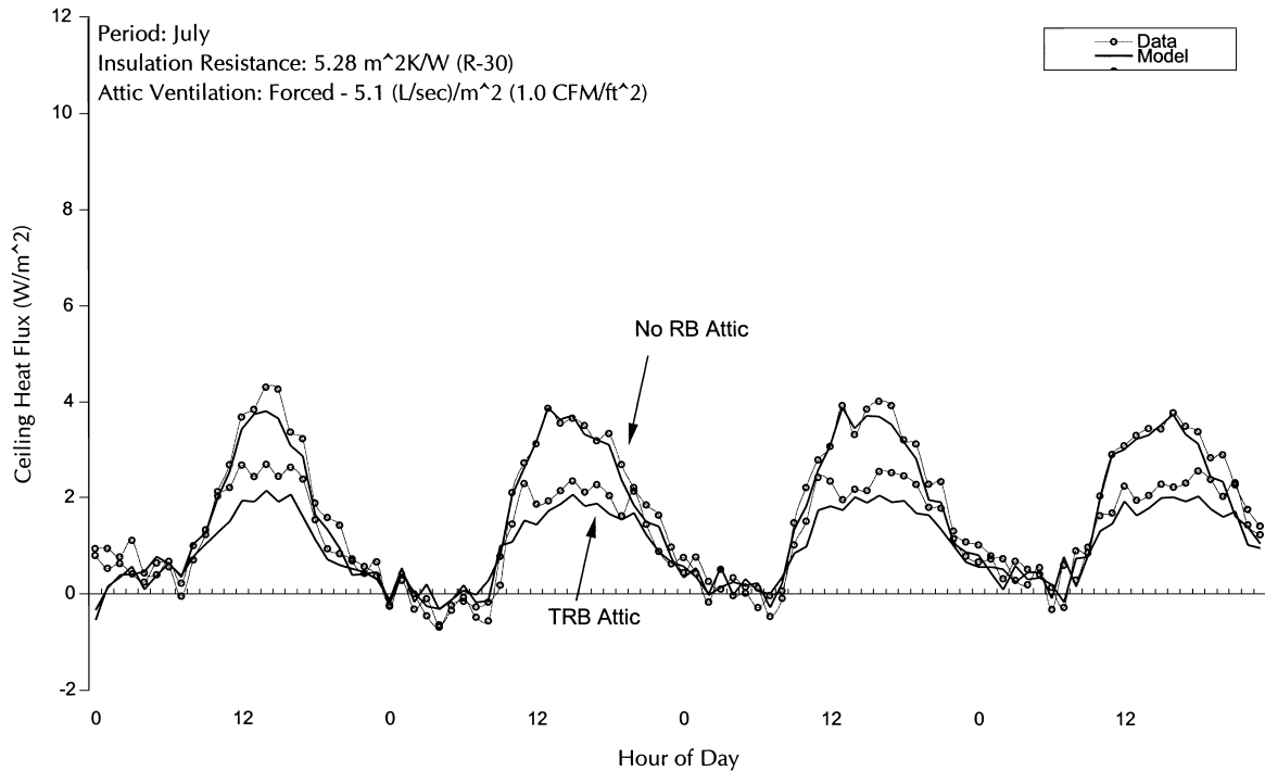
Fig. 7. Ceiling heat fluxes (TRB case, insulation resistance: 5.28 m 2 K/W, R-30; with attic airflow rate: 5.1 l/s/m 2 , 1.0 CFM/ft 2 ).
