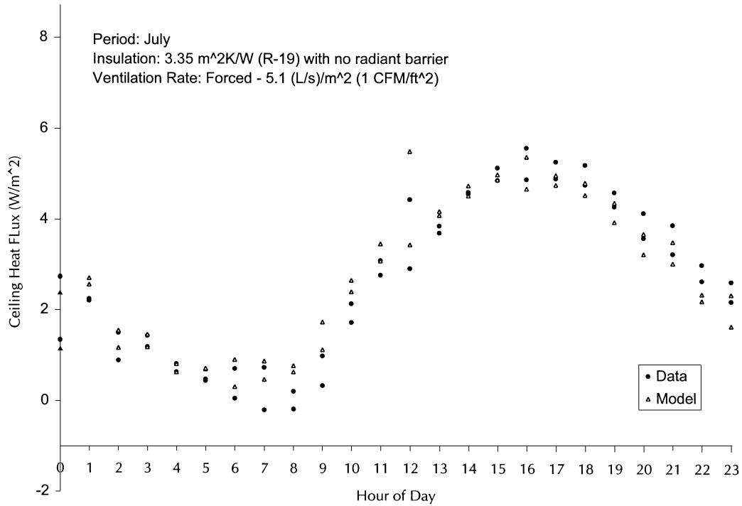
Fig. 4. Measured and predicted heat fluxes (no-RB-case, insulation resistance: 3.35 m 2 K/W, R-19).
