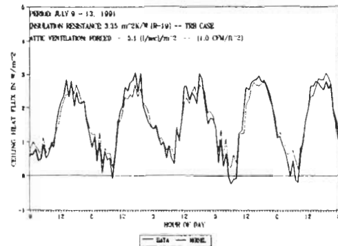
Figure 3. Model Results: ceiling heat fluxes (TRB case, insulation level: R-19; with attic airflow rate: 1.0 CFM/R 2 )
